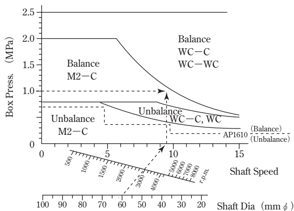
Speed-Pressure Limit
